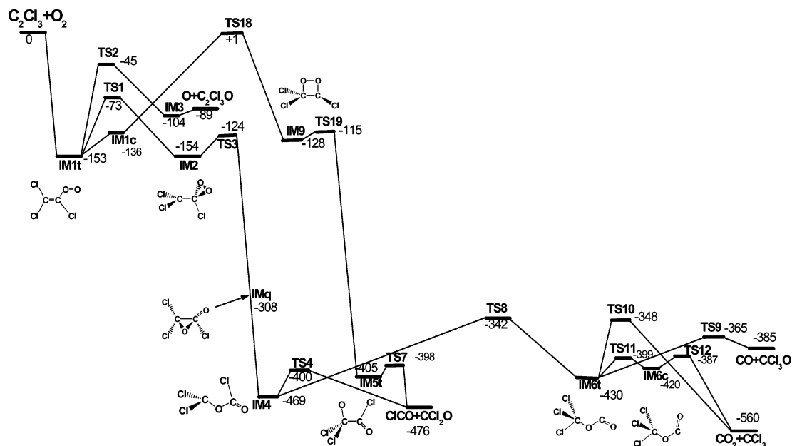
Figure 6. Energy diagram of the C_2Cl_3 + O_2 reaction paths. 4 The indicated energies (in kJ/mol) are obtained at the G3MP2//B3LYP/6-311G(d,p) level of theory. All the energies given are relative to the reactants, and structures of crucial reaction intermediates are shown too.
